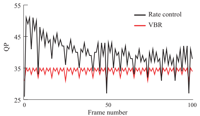
Fig. 3. QP values for the first 100 frames of the Boxing test sequence which correspond to the rate obtained with QP value 31 for VBR. QP values used by rate control are denoted with black, while QP values associated with the random access SOP are depicted with red.
