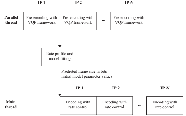
Fig. 6. Block diagram of the proposed approach.
