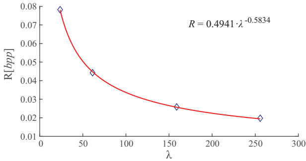
Fig. 1. R - \lambda curve for Manege test sequence. The sequence was encoded using 4 QP values (22, 27, 32, and 37) and obtained rates are denoted as blue diamonds. Fitted R - \lambda curve is depicted in red.
