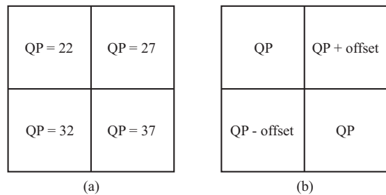
Fig. 5. Variable QP pattern used within a frame for (a) intra frames, (b) inter frames. Each square represents one CTU.
