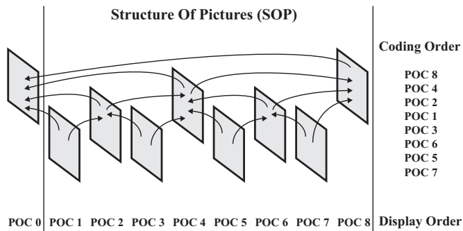
Fig. 2. Random access Structure Of Pictures (SOP) used in the experiments.
