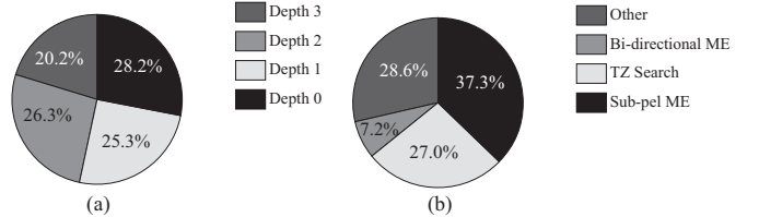
Fig. 4. Percentage of total encoding time spent on testing different coding unit depths (a); and distribution of prediction tasks when the CU depth is equal to zero (b).
