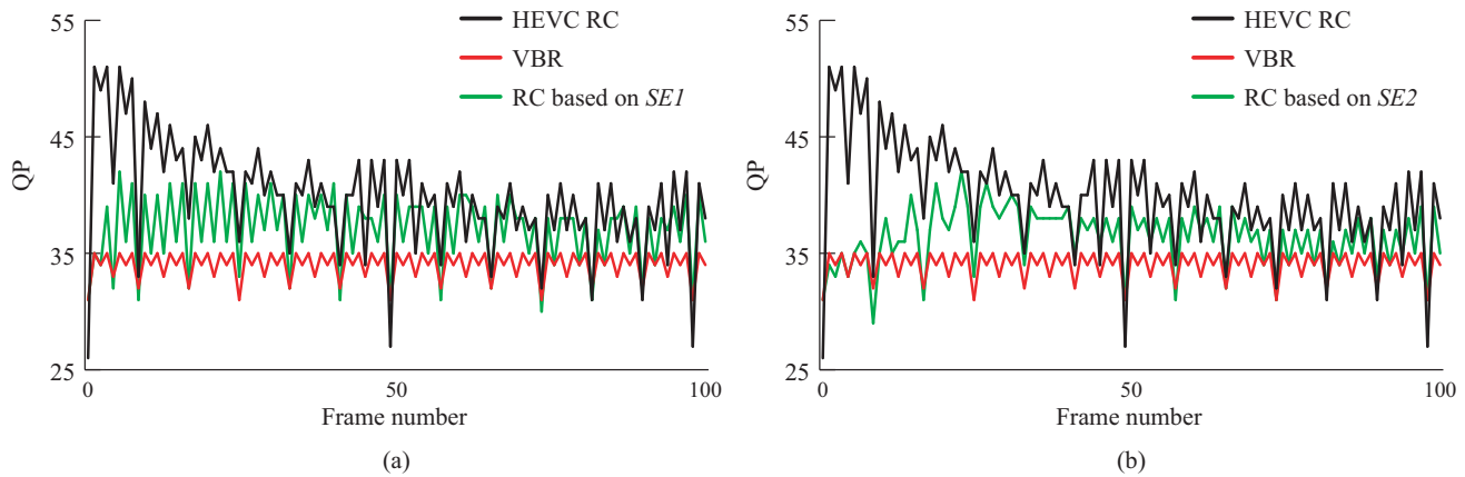
Fig. 7. QP values for the first 100 frames of the Boxing test sequence which correspond to the rate obtained with QP value 31 for VBR. QP values for the VBR configuration are depicted with red, QP values used by the state-of-the-art HEVC rate control are denoted with black, while QP values used by the proposed rate control method based on SE1 (a) and SE2 (b) are denoted with green.
